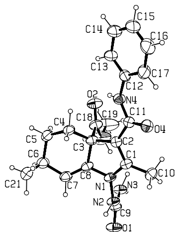
Figure 1. A view of the asymmetric unit of 4f , showing the labelling of the non-hydrogen atoms.
